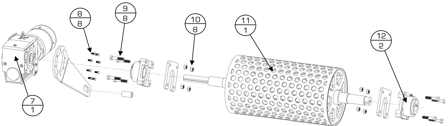
Screen Roller ASM
