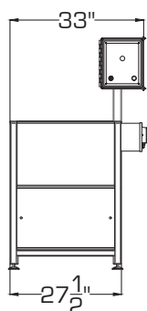
WNW 150
